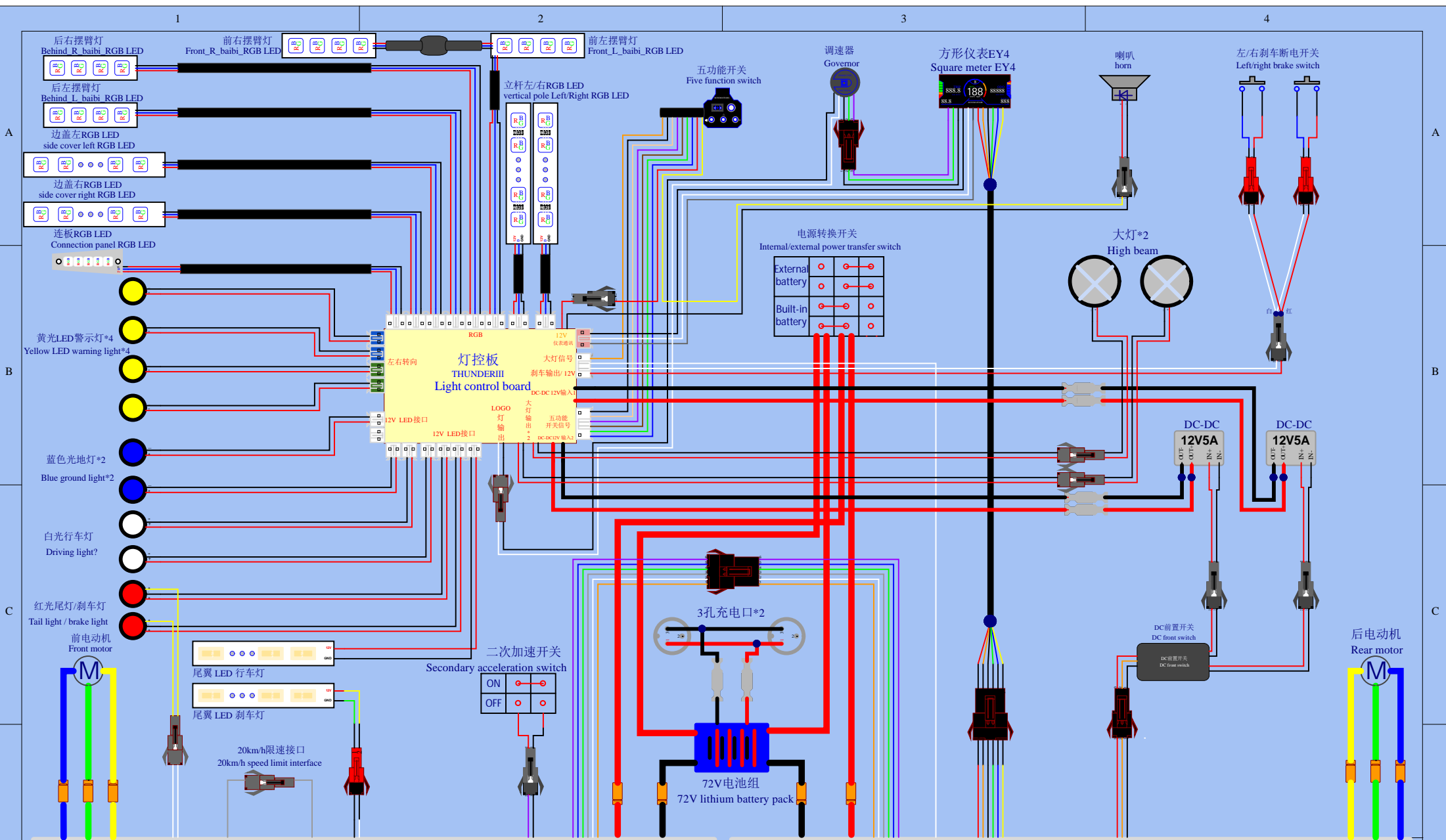
DT-THUNDERIII型直流无刷前电机控制器 (A) DT-THUNDERIII type DC brushless front motor controller (A)
